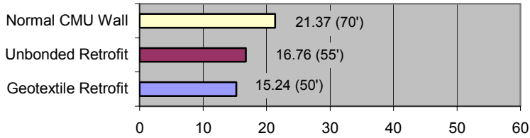
CMU Wall Damage - With Blast Wall Meter (ft)
