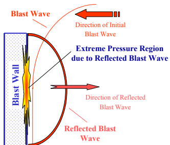
Figure 14: Reflected Pressure
