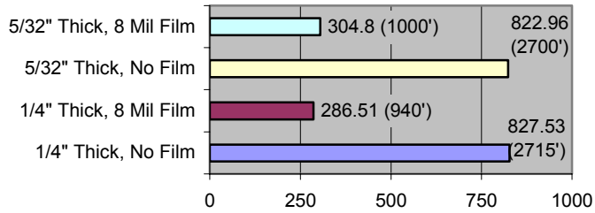
1219.20 mm x 1524 mm (48" x 60") Window Hazard Distances in Meters (ft) - No Blast Wall
