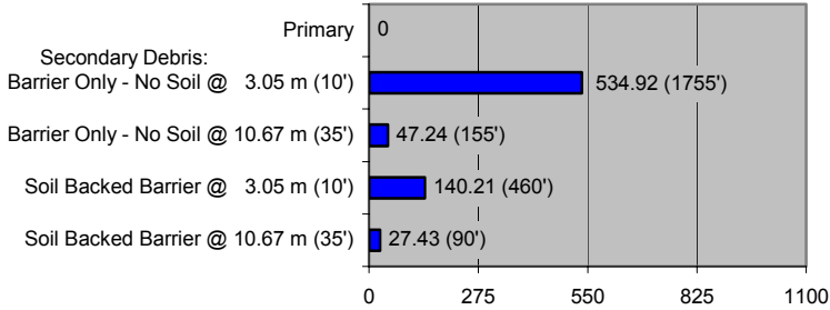
Debris Hazard Distances - Meter (ft)
