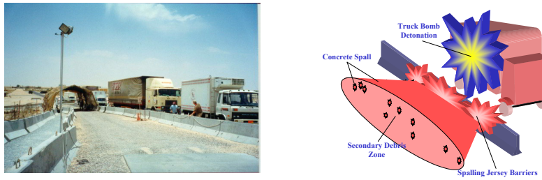
Figure 21: Fragmenting Jersey Barriers
