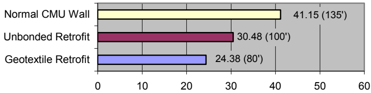
CMU Wall Damage - No Blast Wall Meter (ft)
