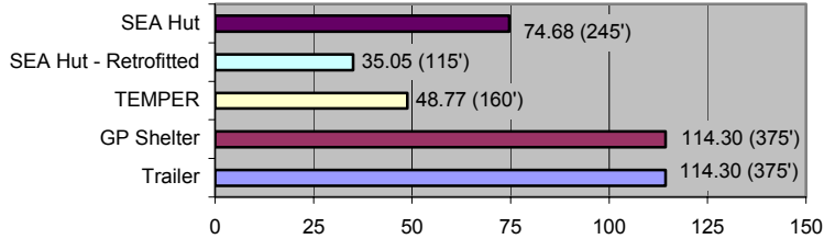
Expeditionary Structure Damage - No Blast Wall Meter (ft)
