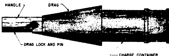
Figure 4-5. Shaped charge hand grenade.
