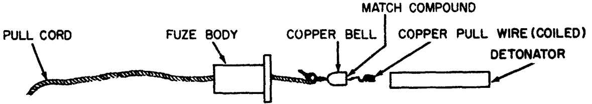
FUZE COMPONENTS
