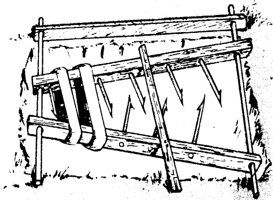
Figure 4-51. Sideways closing trap.
