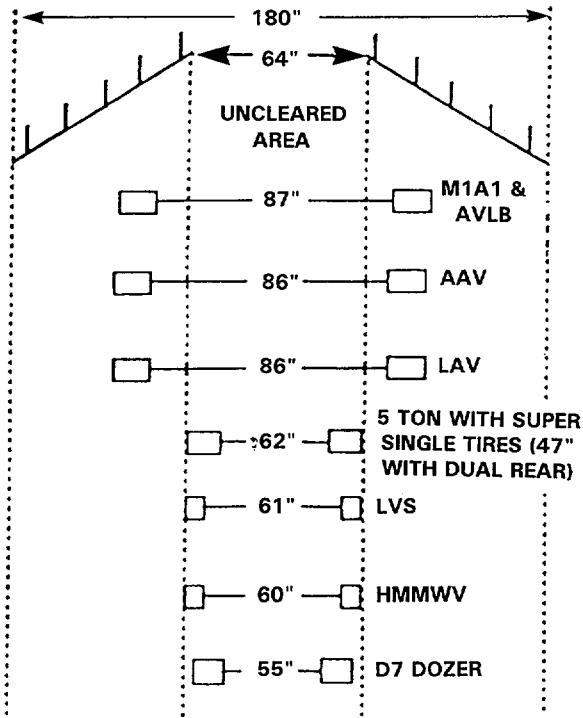
Figure B-17. TWMP Cleared Path.
