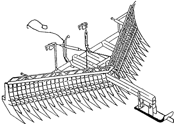
Figure F-1. Full-Width Mine Rake.
