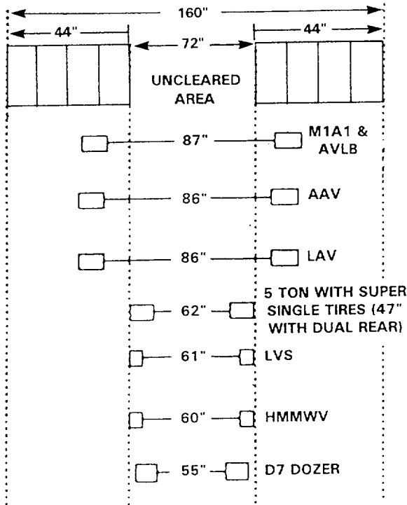
Figure C-4. Mine Roller Path.
