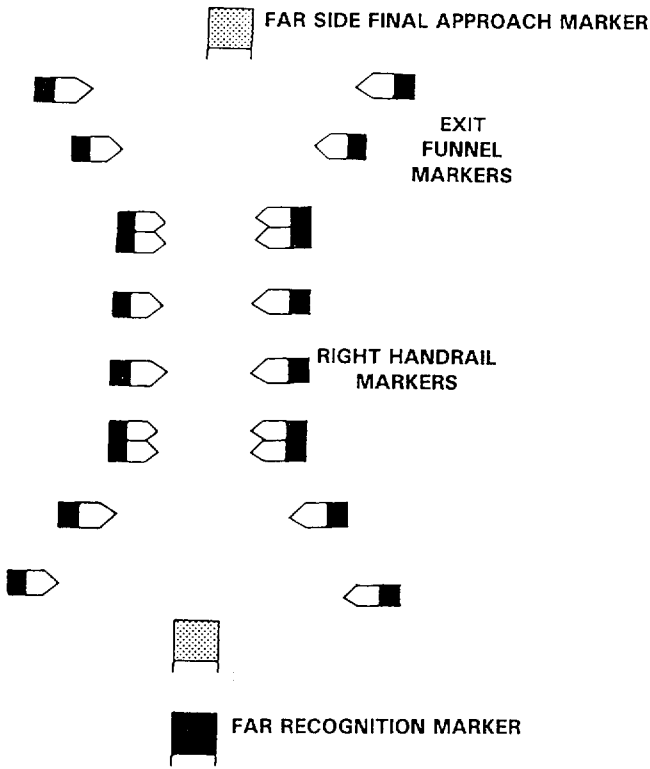
Figure 7-7. Intermediate Lane Marking.
