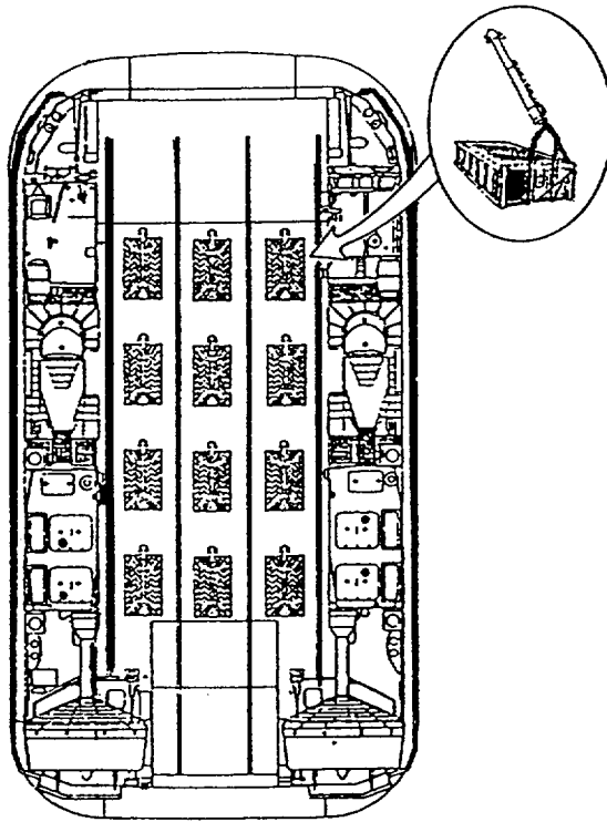
Figure E-6. LCAC Preloaded with 12 MICLICs.
