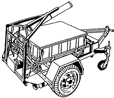
Figure B-15. MK 2 Mine Clearance System.
