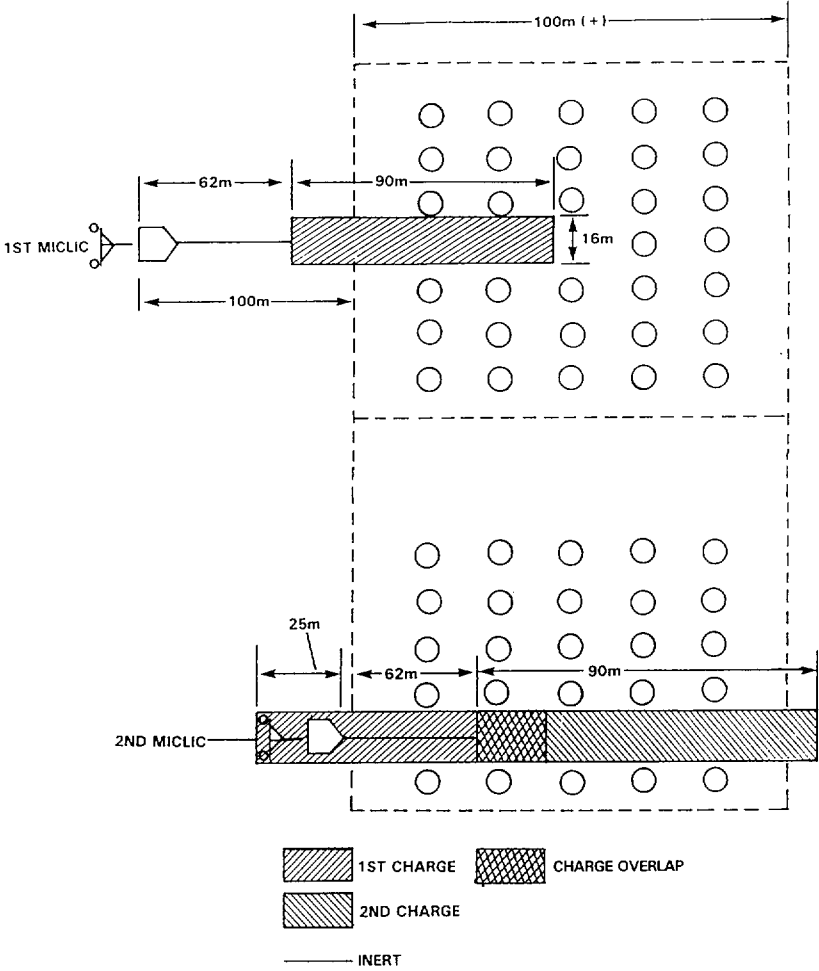
Figure B-13. Use of One or More MICLICs.
