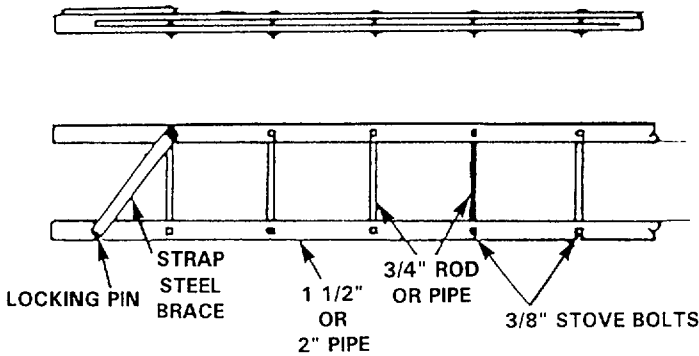
Figure B-1. Assault Ladder.
