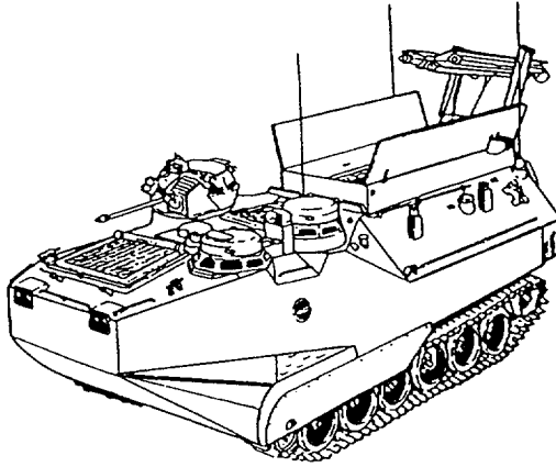
Figure B-14. MK 1 Mine Clearance System.
