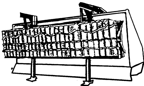
Figure B-9. Blade-Placed Explosive Charge.
