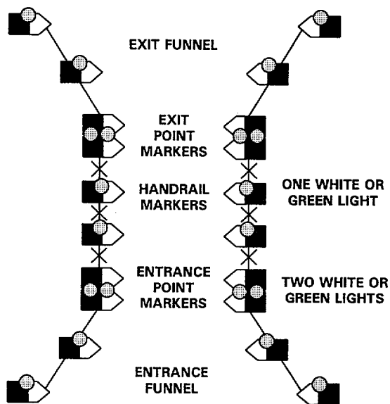
Figure 7-11. NATO Marking for Limited Visibility.
