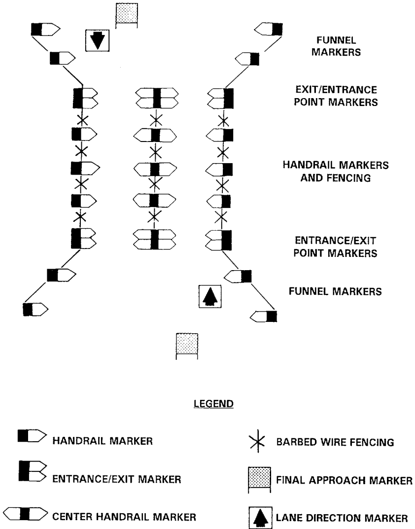
Figure 7-10. NATO Full Lane Marking.
